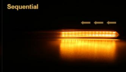
Sequential
