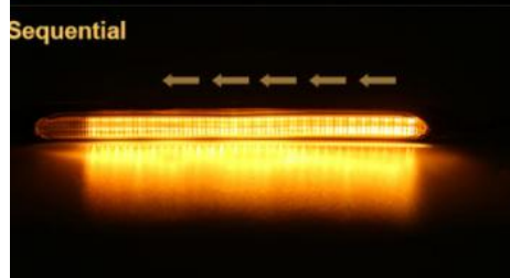
Sequential
